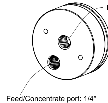
Feed/Concentrate port female thread options:
