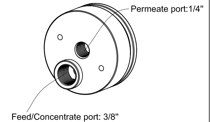
Feed/Concentrate port female thread options:
